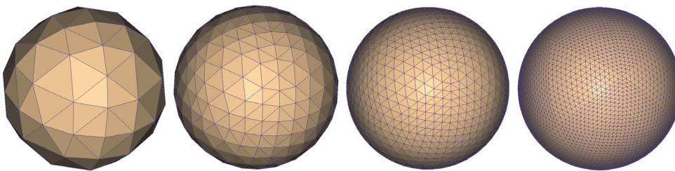
FIG. 3. The discretization of the sphere, from left to right: n_V = 66, 258, 1026, 4098 .
