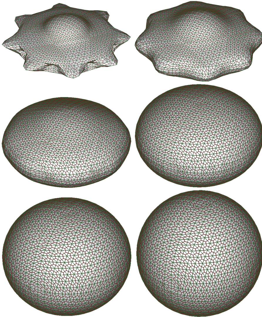
FIG. 10. Evolution of a discretized cymling-like shape with 1026 grid points, \tau = 7.5e - 4 , the volume preserving mean curvature flow. Both triangle and co-volume mesh are displayed. The selected time steps are n = 0 , n = 10 , n = 40 , n = 100 , n = 250 , n = 1000 . The asymptotically uniform tangential redistribution with \omega = 100.0 was used.
