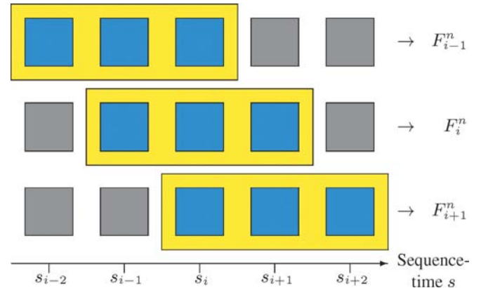
Fig. 9. The block solver considers in each step of the inner frame loop always only three successive images of the sequence. This corresponds to the fact that the resulting system matrix has a 3-band block-structure
