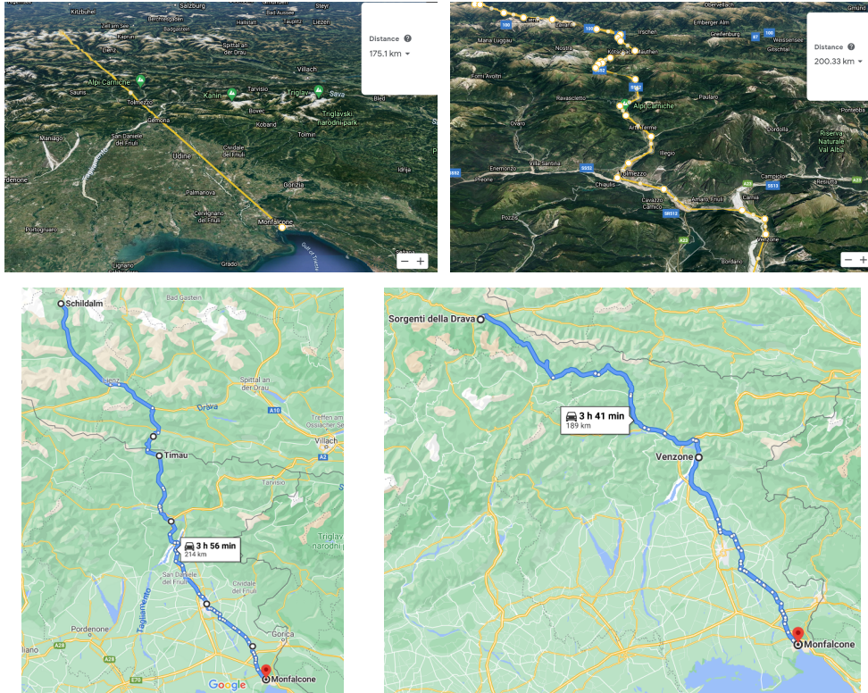
FIGURE 1.2. Distances to the recess of Adriatic (Monfalcone). Left up: geodesic line distance from the source of Tauernbach in the High Tauern (175 km). Right up: geodesic distance from the source of the Tauernbach through the passable valleys (200 km). Left down: distance from the source of the Tauernbach by local roads (214 km). Right down: distance from the source of the Drava river by local roads (189 km). Upper images were created by the Google Earth application while bottom images by the Google Maps application.
